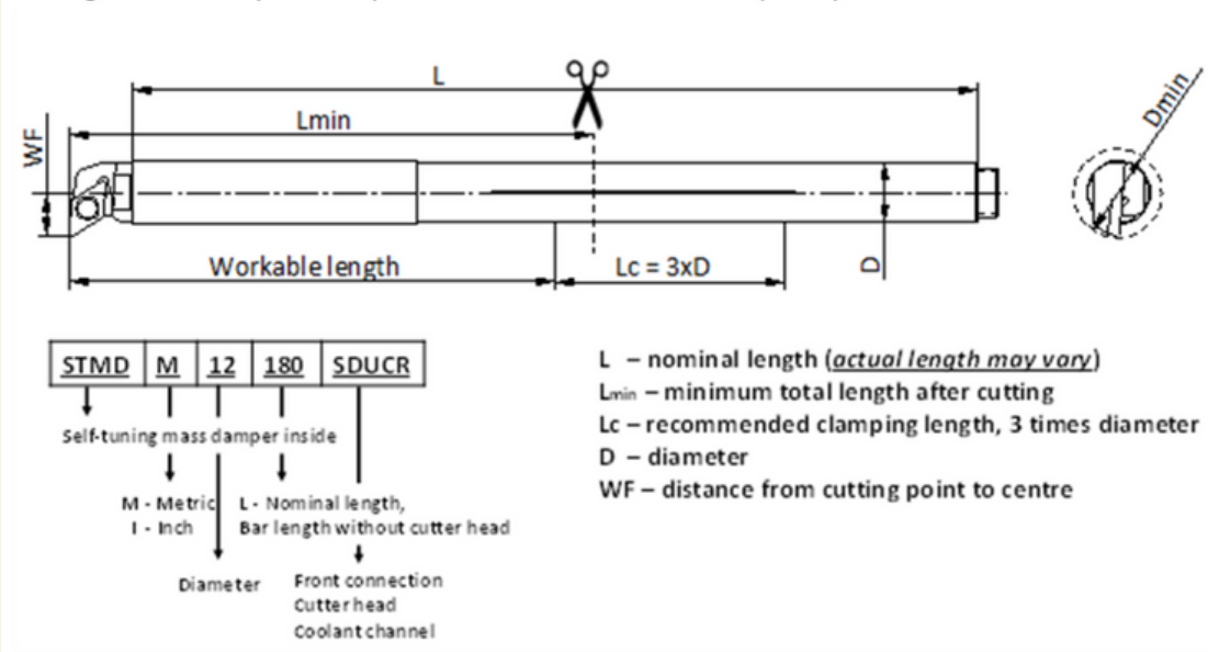
Straight holder (8-12xD) with fixed cutter heads (Inch)
